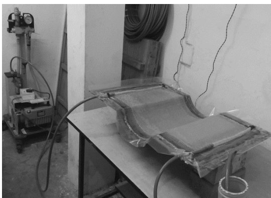
(a) Vacuum bagging technique
